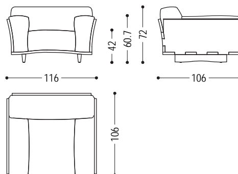
NUDO ARMCHAIR
